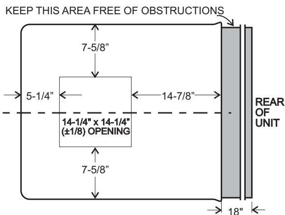
FIG. 1 AIR CONDITIONER/HEAT PUMP DIMENSIONS (On Top of Vehicle)
