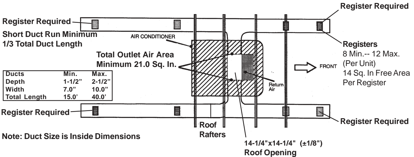
FIG. 4 Duct Size And Requirements For 3308120.XXX Genesis Air Filtration System
